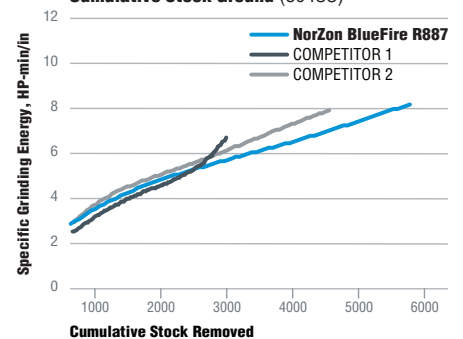
Specific Grinding Energy vs. Cumulative Stock Ground (304SS)
